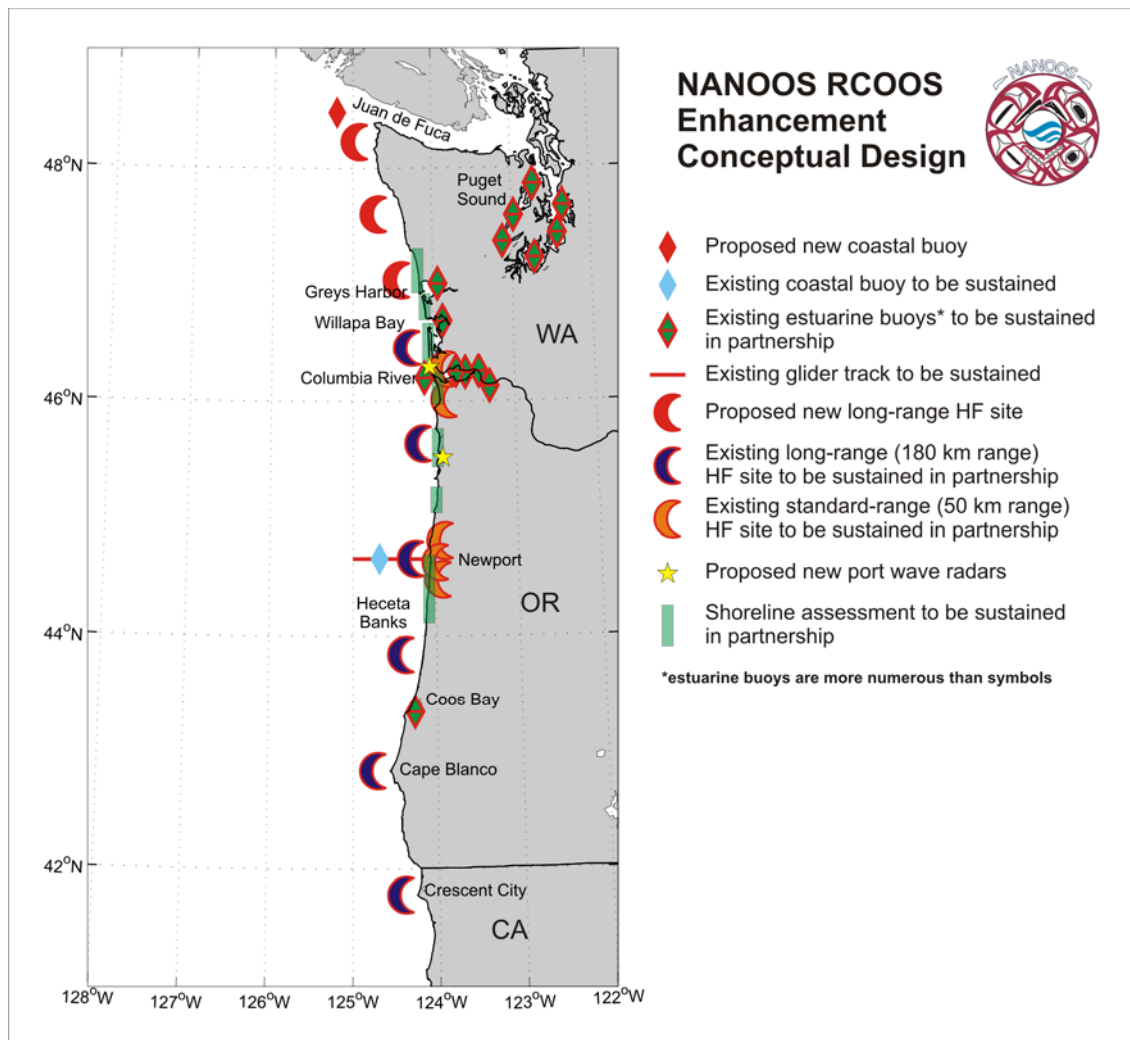
Figure 1. Conceptual design for NANOOS RCOOS enhancements for observing assets to be funded from this proposed effort.
