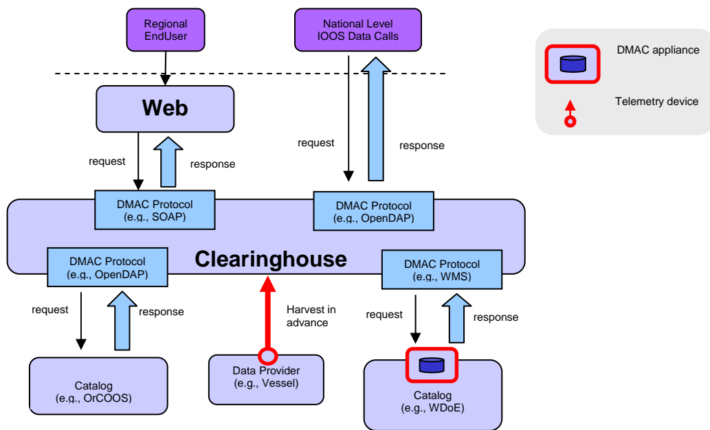
Figure 2. Chart showing NANOOS DMAC system of systems centered around a Clearinghouse and Web Portal. Requests may be served directly by the Clearinghouse or forwarded to remote catalogs. Some catalogs will be "DMAC-enabled" by deployment of a DMAC appliance.
